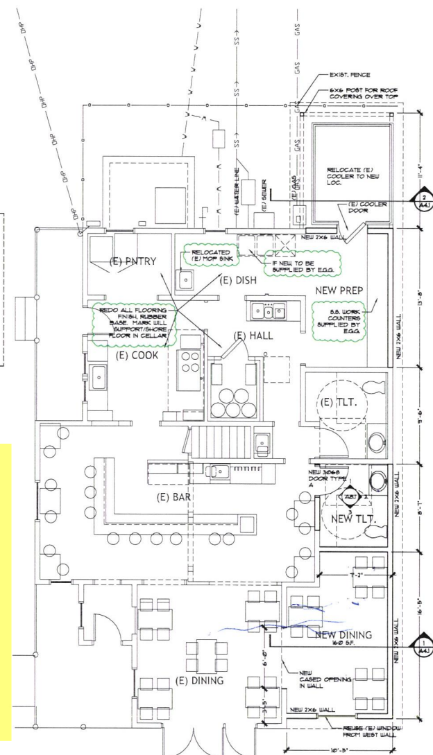
2 A2.1 PROPOSED FLOOR PLAN SCALE: 1/4" = 1'-0"
