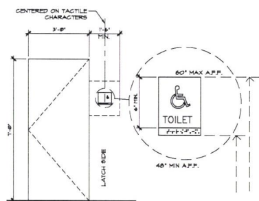
3 DOOR SIGN DETAIL A2.1 SCALE: 1/2" = 1'-0"
