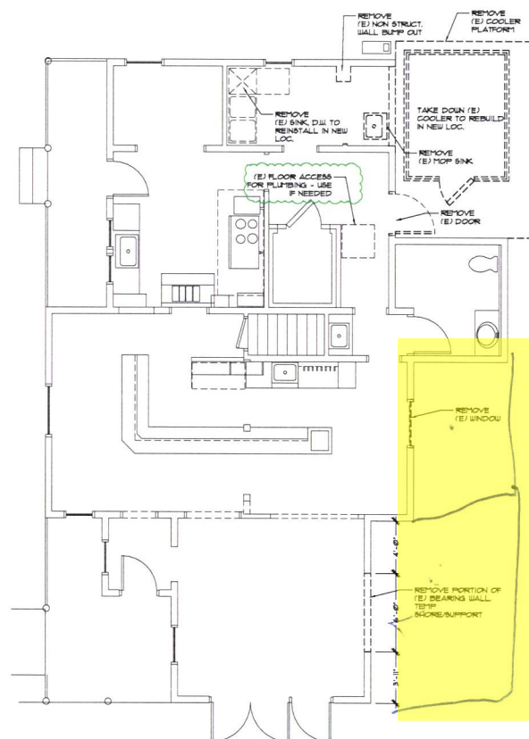
EXISTING - DEMO FLOOR PLAN SCALE: 1/4" = 1'-0"
