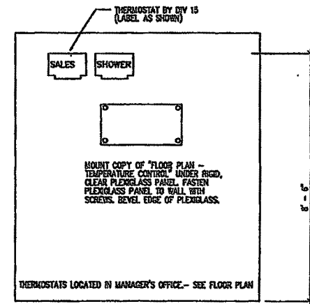
2 THERMOSTAT INSTALLATION SCALE: NONE
