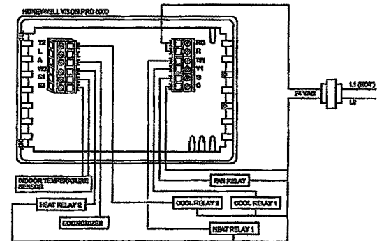
4 TYPICAL 2H/2C MULTISTAGE THERMOSTAT WIRING SCALE: NONE
