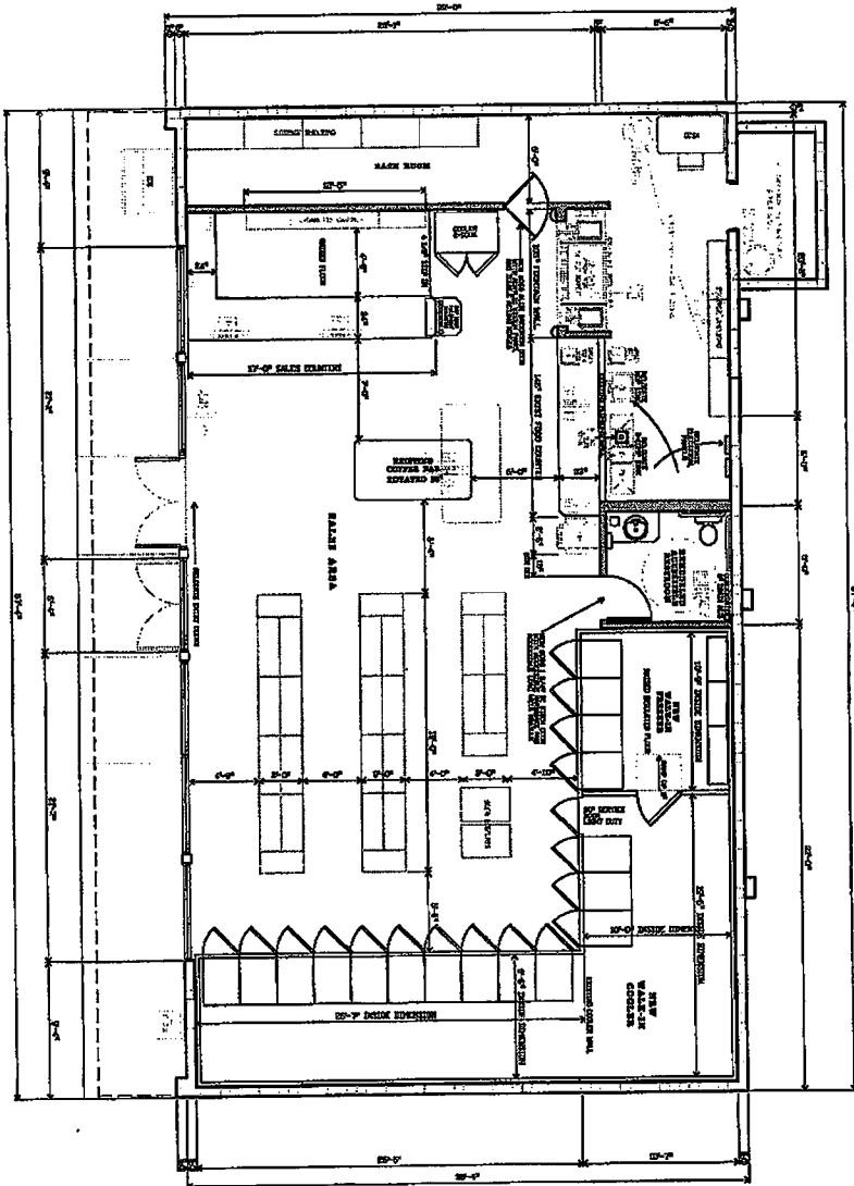
Remodel Floor Plan 1/4"
