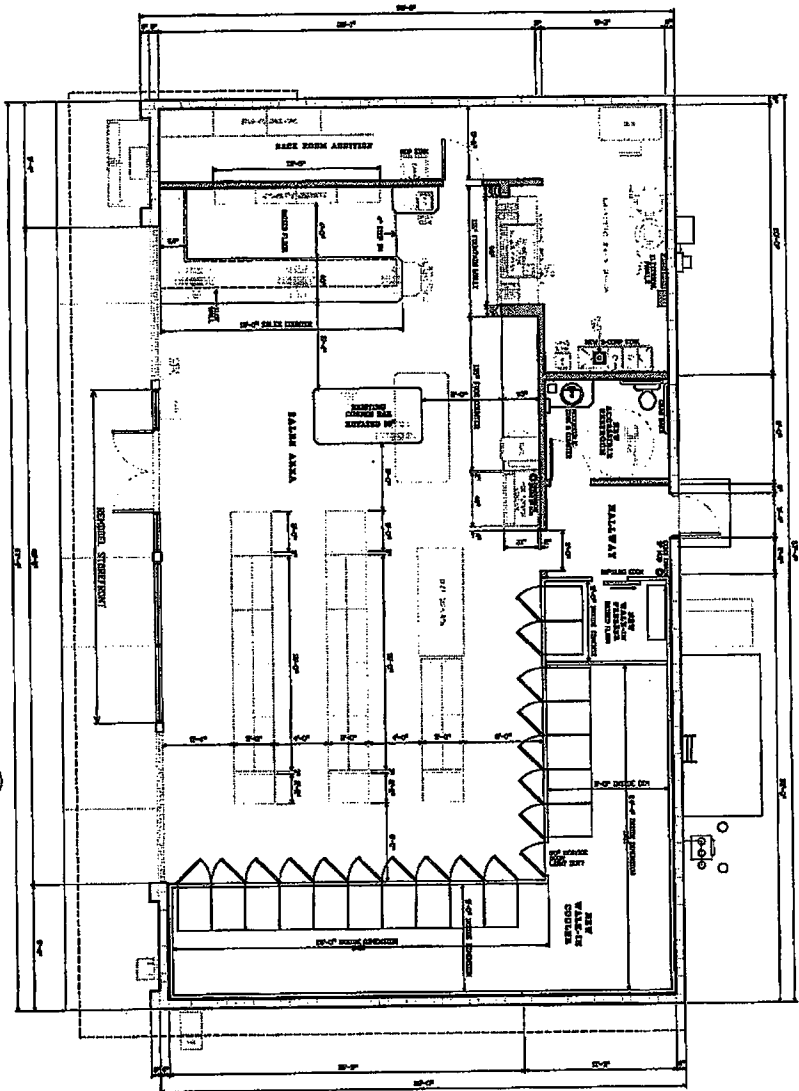
Remodel Floor Plan 1/4"
