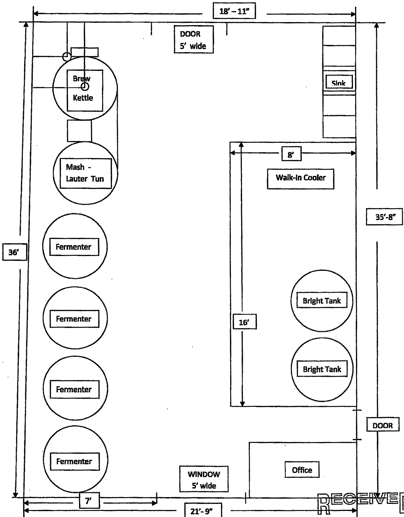
Brewery Floor Plan
