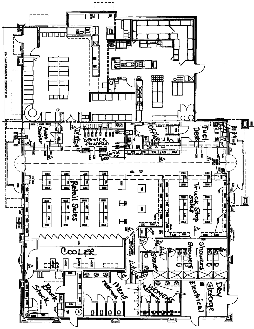
A EQUIPMENT FLOOR PLAN SCALE 1/8" = 1'-0"
